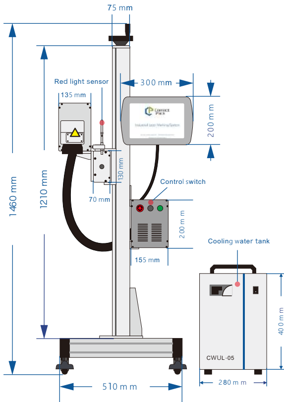
FRONT OF THE DEVICE
